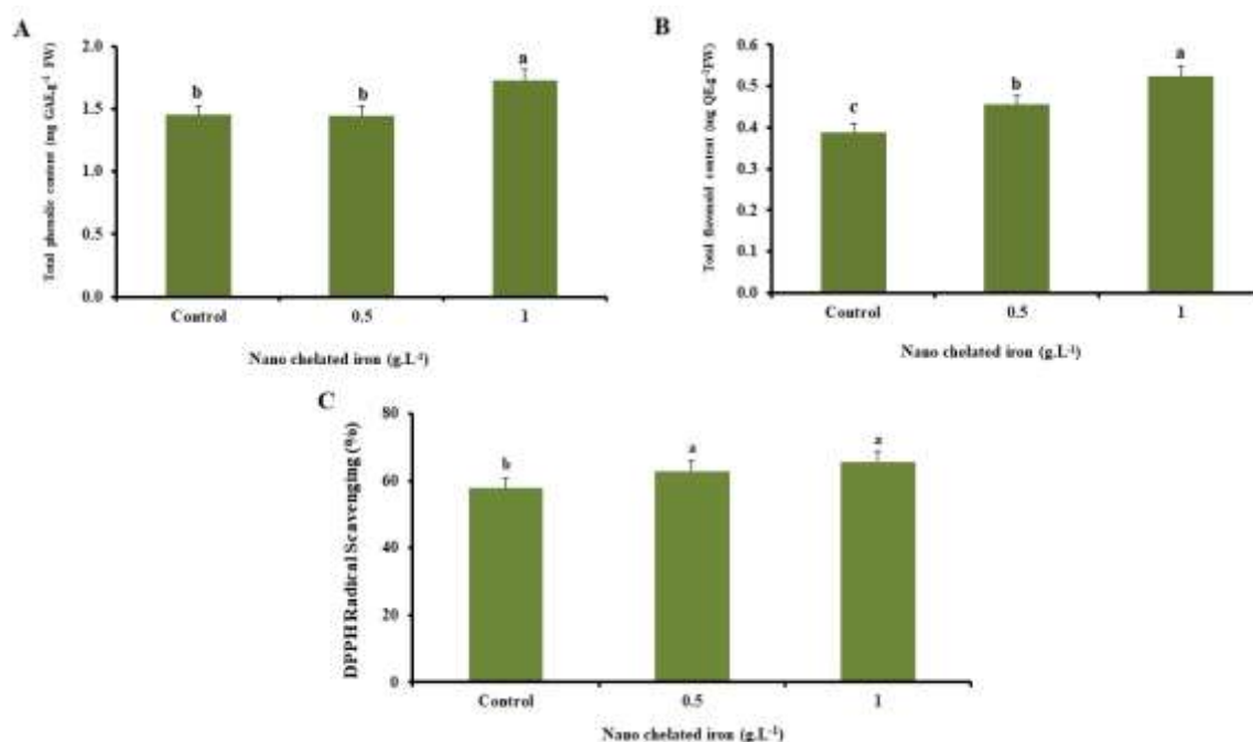
Figure 1- Effects of different concentrations of nano chelated iron on A) Total phenolic content, B) Total flavonoid content, C) DPPH Radical Scavenging
