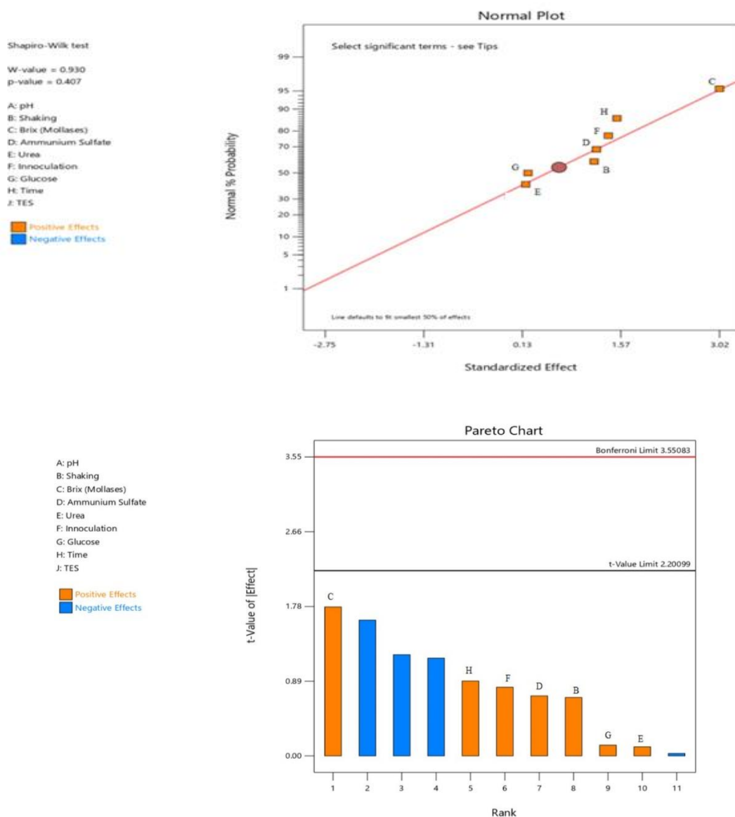
Fig. 3. The normal distribution curve of plackett burman's plot related to the screening of independent variables influencing P. polymyxa biomass (Normal plot and Pareto chart).
