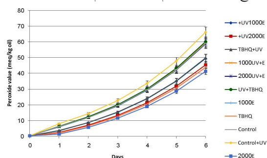
Fig 1 Peroxide value of different corn oil sample during 6 days storage at 60 °C
