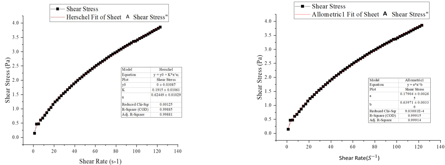
Figure2. Shear stress diagram in terms of shear rate in treatment with 1% of fiber (pseudoplastic fluid)
