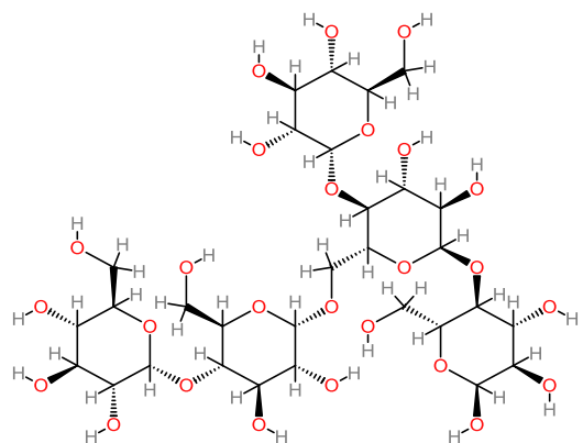
Amylopectin ( C_{30}H_{52}O_{26} )
