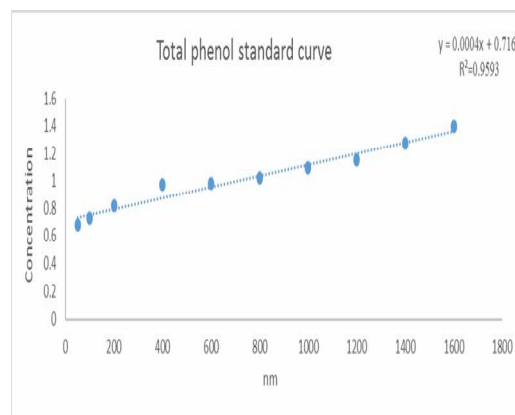
Fig 1 Standard gallic acid curve in total phenolic compounds test
