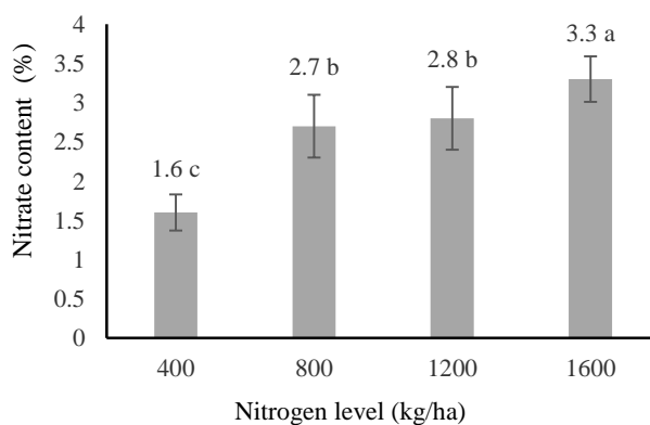
Figure (2) Mean comparison of nitrate content (%) of treatments (Different letters show significant difference at 5 % probability level)
