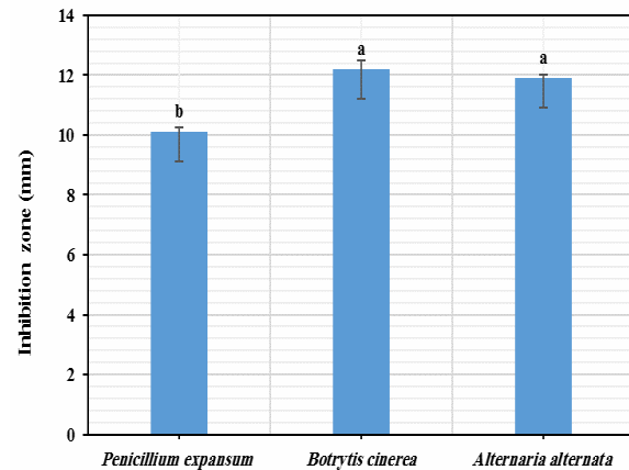
Fig 3 Antifungal activity of Salvia mirzayanii essential oil, according to disk diffusion agar test.
