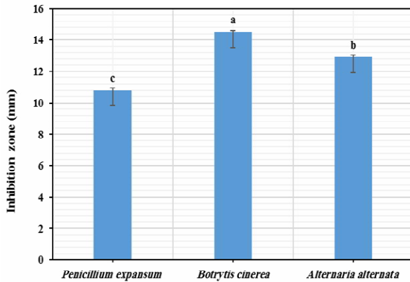
Fig 4 Antifungal activity of Salvia mirzayanii essential oil, according to well diffusion agar test.
