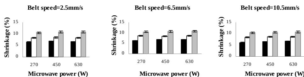
Fig 5 Shrinkage values of almond kernels in semi industrial continuous dryer (■45°C, □60°C and ■75°C)
