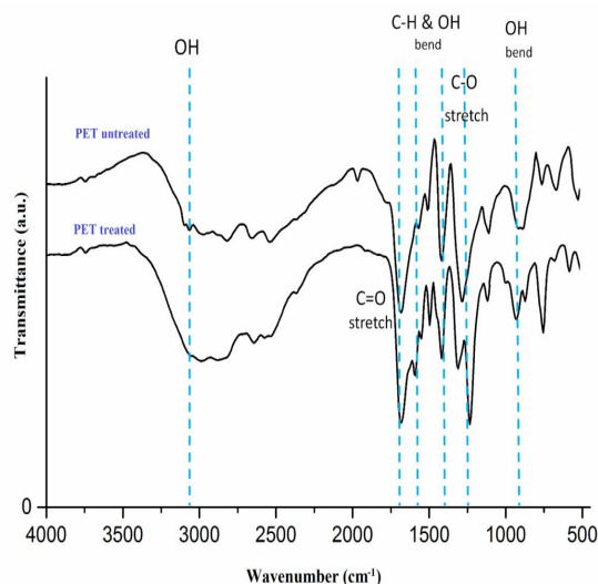
Fig 6 ATR-FTIR of the PET films: (a) untreated PET (b) plasma-treated PET
