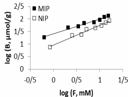
Fig 3 Freundlich binding isotherm of optimized MIP and its corresponding NIP (log-log format).
