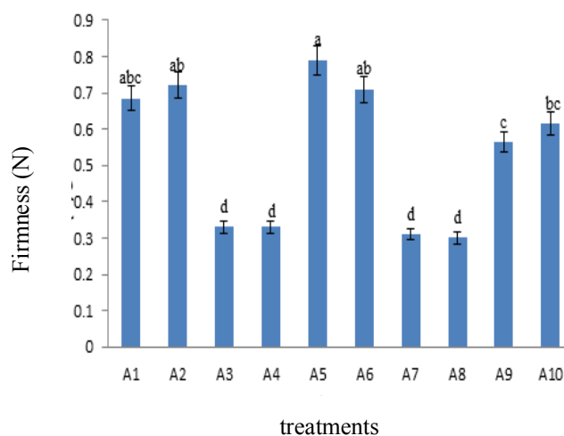
Fig 6 The results for firmness of ice cream samples containing different percentages of fat , different homogenation pressures and different types of emulsifier
