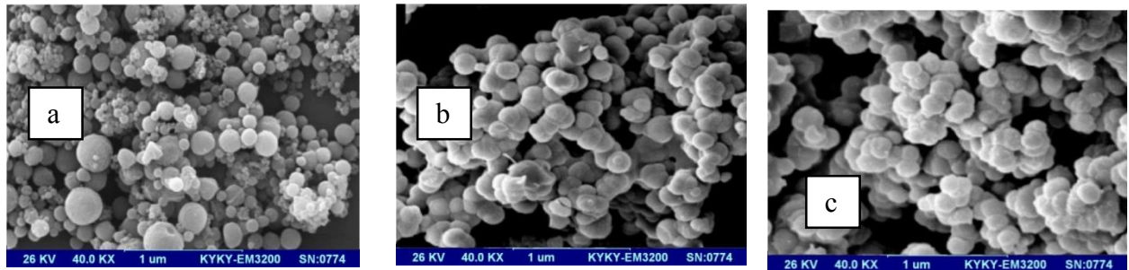
Illustration 1 SEM images of (a) basil coating containing 1% black cumin EO, (b) basil coating containing 1% 1.5% black cumin EO and (c) basil coating containing 2% black cumin EO
