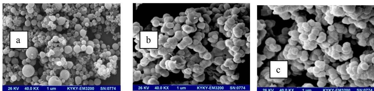
Illustration 1 SEM images of (a) basil coating containing 1% black cumin EO, (b) basil coating containing 1.5% black cumin EO and (c) basil coating containing 2% black cumin EO
