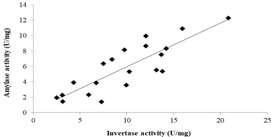
Fig 3 The regression curve for specific activity of amylase versus invertase of 20 Iranian honey samples.
