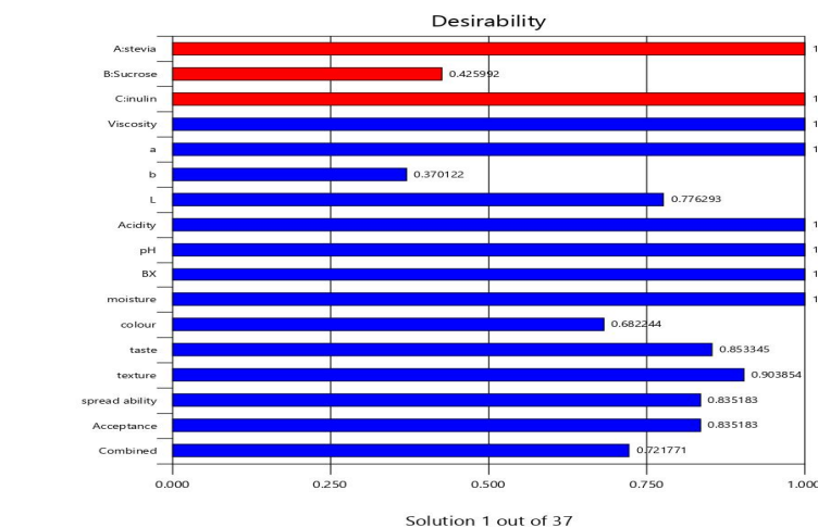
Fig 8 Optimal sample chosen by RSM
