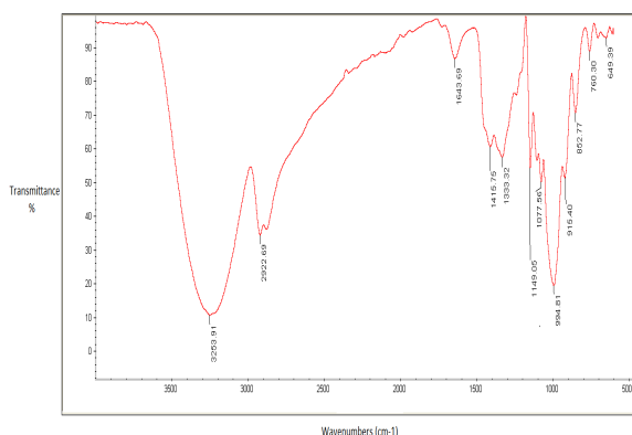
Fig 8 FTIR diagram of the Potato starch film contains 1.5 per cent of eucalyptus oil.
