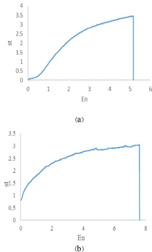
Fig 4 Stress –Elongation of fibers (a) free of Artemisia Extract, (b) loaded with Artemisia Extract
