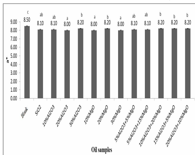
Diagram 9 The red color of bleached soybean oil samples using 1% of adsorbent consisting of different percentages of SiO 2 , Al 2 O 3 and MgO
