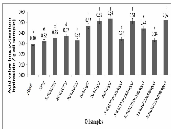
Diagram 3 The acid values of bleached soybean oil samples using 1% of adsorbent consisting of different percentages of SiO 2 , Al 2 O 3 and MgO
