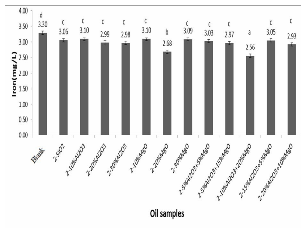
Diagram 14 The iron contents of bleached soybean oil samples using 2% of adsorbent consisting of different percentages of SiO 2 , Al 2 O 3 and MgO
