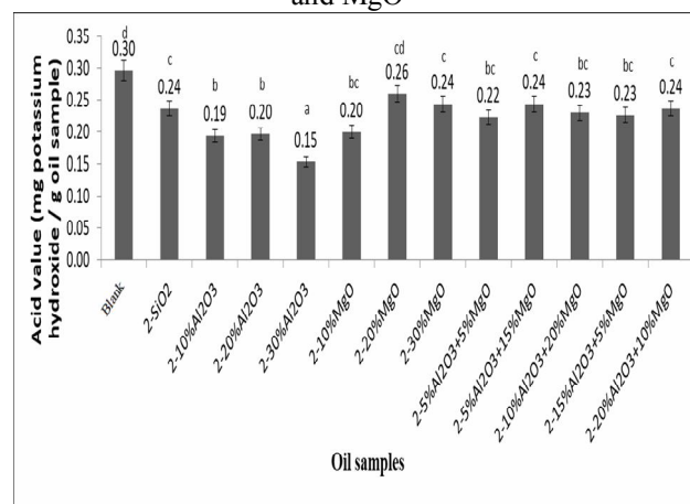
Diagram 4 The acid values of bleached soybean oil samples using 2% of adsorbent consisting of different percentages of SiO 2 , Al 2 O 3 and MgO
