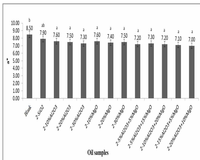
Diagram 10 The red color of bleached soybean oil samples using 2% of adsorbent consisting of different percentages of SiO 2 , Al 2 O 3 and MgO
