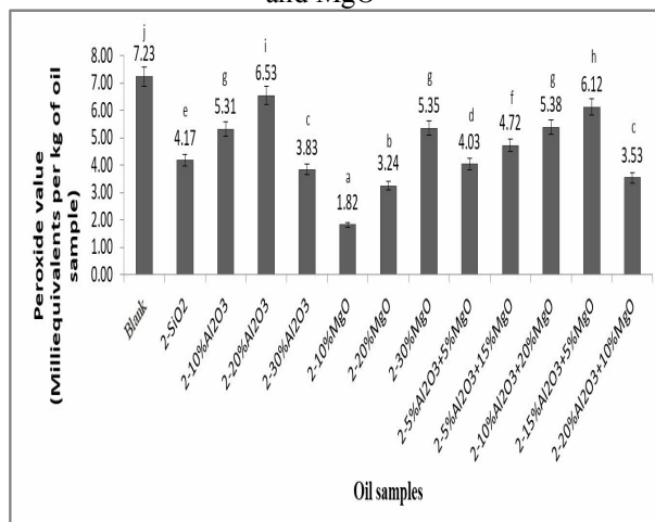
Diagram 2 The peroxide values of bleached soybean oil samples using 2% of adsorbent consisting of different percentages of SiO 2 , Al 2 O 3 and MgO
