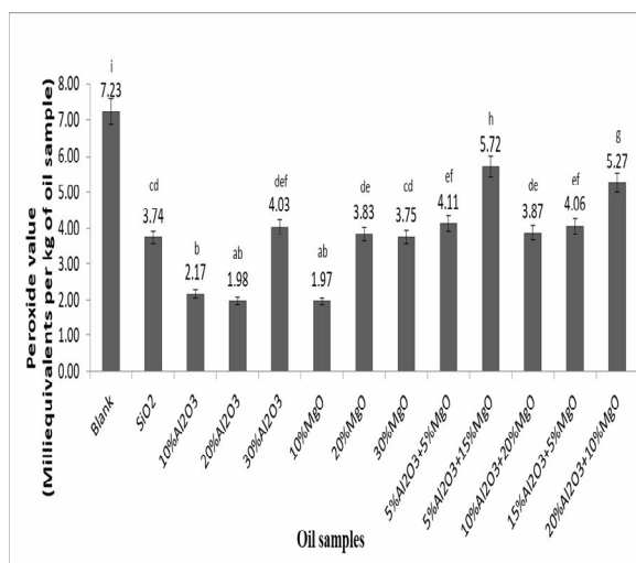
Diagram 1 The peroxide values of bleached soybean oil samples using 1% of adsorbent consisting of different percentages of SiO 2 , Al 2 O 3 and MgO
