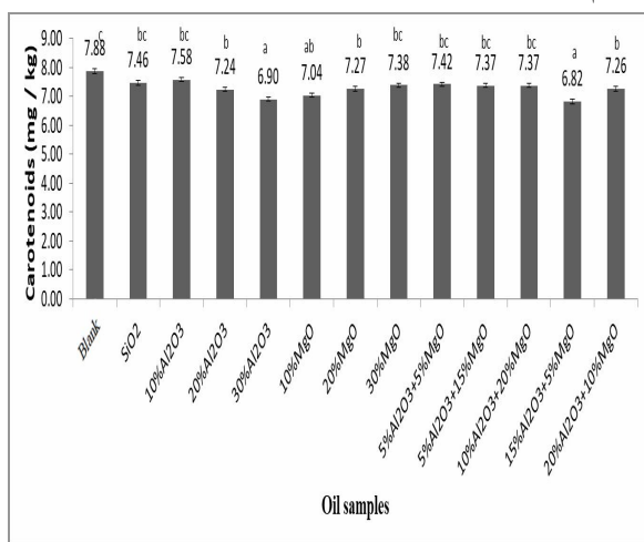
Diagram 7 The Carotenoid values of bleached soybean oil samples using 1% of adsorbent consisting of different percentages of SiO 2 , Al 2 O 3 and MgO
