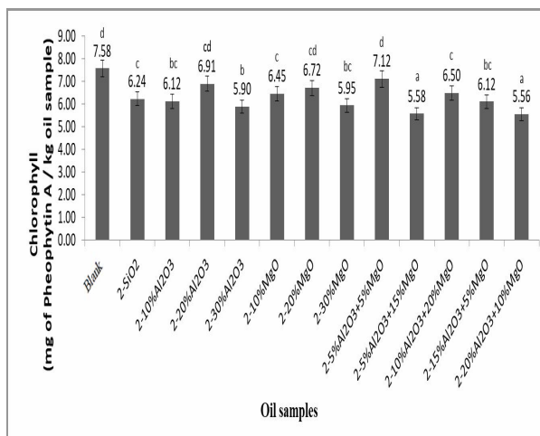
Diagram 6 The chlorophyll values of bleached soybean oil samples using 2% of adsorbent consisting of different percentages of SiO 2 , Al 2 O 3 and MgO
