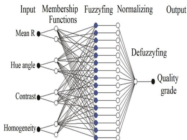
Fig 2 ANFIS structure.
