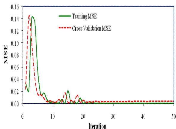
Fig 5 Mean square error (MSE) values as a function of the learning iterations number during training and validation by ANN
