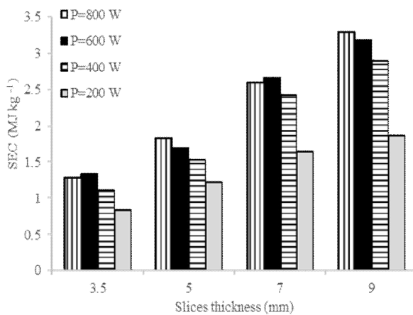
Fig 1 Average specific energy consumption (SEC) of microwave drying process of potato slices
