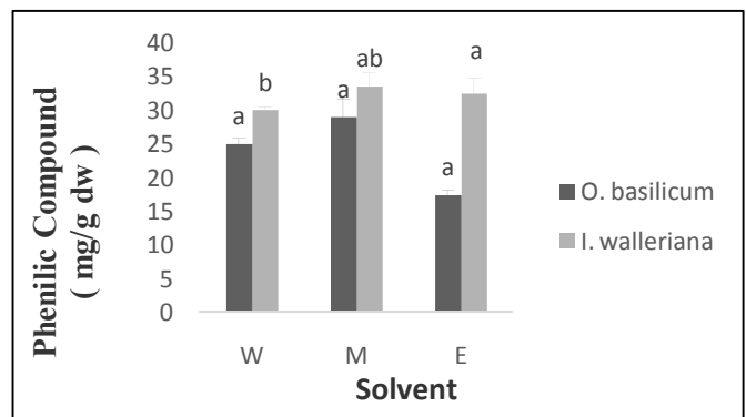
Fig 1 Phenolic content of Ocimum basilicum and Impatiens walleriana extracts (Water: W, Methanol: M, Ethanol: E) using water bath method. The values with different superscript letters in a column are significantly different (p<0.05).
