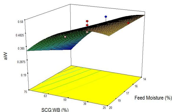
Fig 2 Response surface plot showing the effects of the Ratio of SCG:WB and Feed Moisture on a_w .
