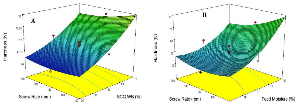
Fig 4 Response surface plot showing the effects of A) the Ratio of SCG:WB and Screw Rate, B) Feed Moisture and Screw Rate on Hardness.
