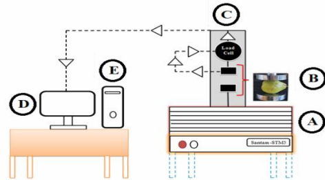
Fig 2 Diagram of pears quasi-static loading
