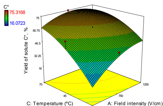
Fig 6 The interaction effect of electric field intensity and temperature on the final solute extraction yield based on CCD. ( t = 255\text{ min} , n = 45 )
