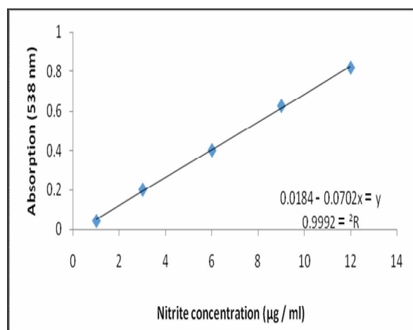
Fig 1 Standard curve prepared based on different amounts of sodium nitrite in standard solutions
