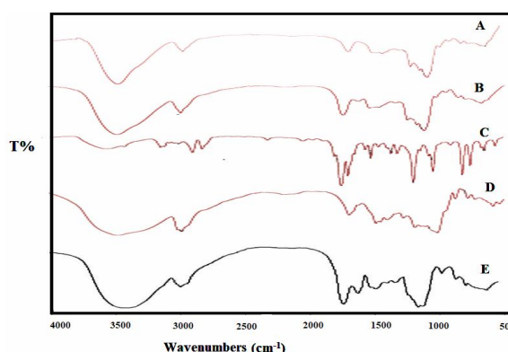
Fig 4 FT-IR (A) \beta -cyclodextrin with essential oil, (B) \beta -cyclodextrin and sodium caseinate with essential oil, (C) cinnamon essential oil, (D) \beta -cyclodextrin, (E) sodium caseinate.
