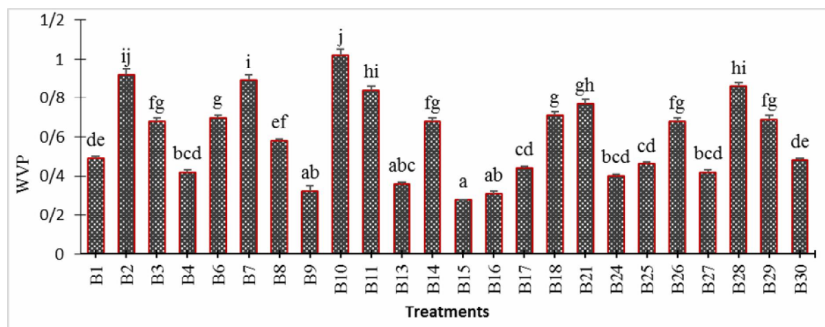
Fig 3 Water vapor permeability of gelatin films produced by investigating the effect of effective factors on extraction.
