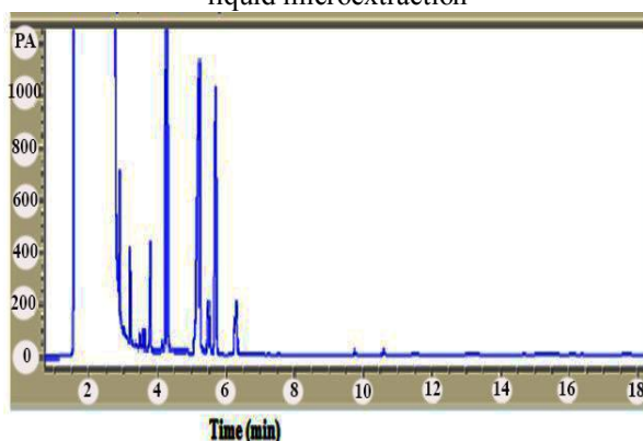
Fig 2 The chromatogram is the essential oil release in yogurt
