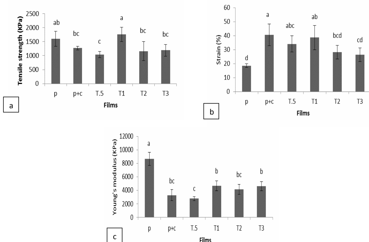
Fig 3 Effect of different amounts of \text{TiO}_2 and carnauba wax on tensile strength (a), strain (b), and young's modulus (c) of pectin-based films (p: pectin, c: carnauba wax, T: \text{TiO}_2\% )
