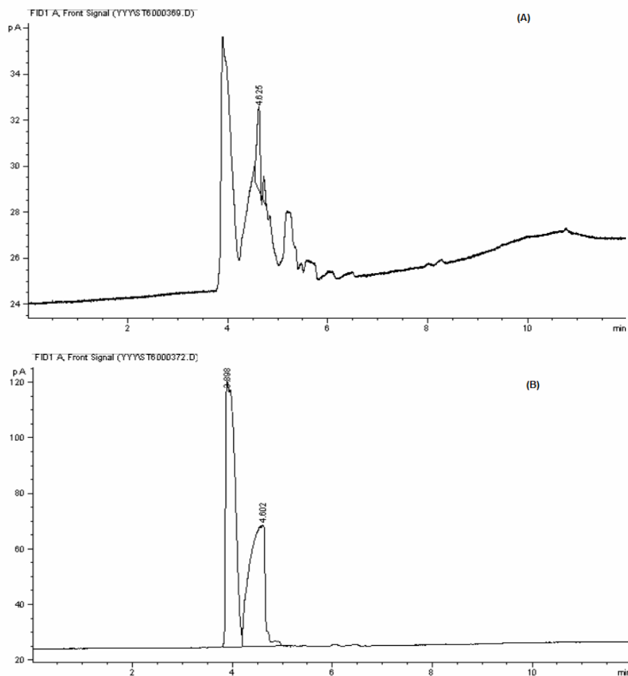
Fig 1 Recorded peaks by detector of gas chromatography for nanoemulsions containing garlic essential oil at fixed ratios (15 % garlic extract) (A) and garlic extract and sunflower oil mixture (B).
