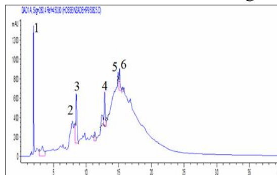
Fig 2 Grape seed extract chromatogram
