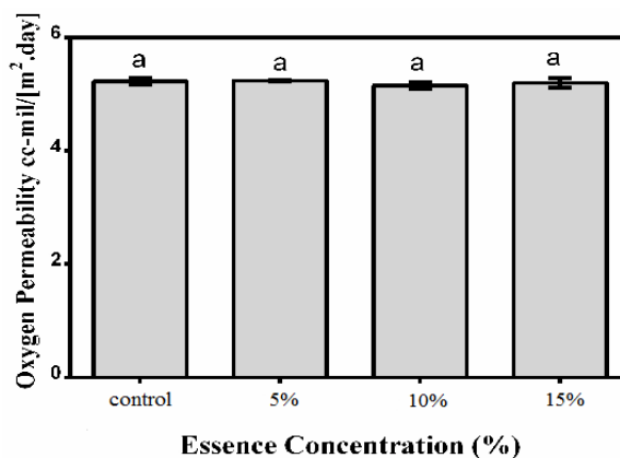
Fig 4 Effect of different percentage of harmal essence on oxygen permeability cc-mil/[m 2 ·day] of SSPS and nanoSiO 2 films. Values are means \pm SE (n = 5). Different letters are significantly different at (P < 0.05).
