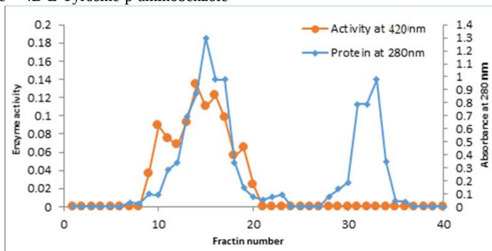
Figure 6: Elution profile of Mirabelle plum PPO by CM-cellulose column (2×25 cm)
