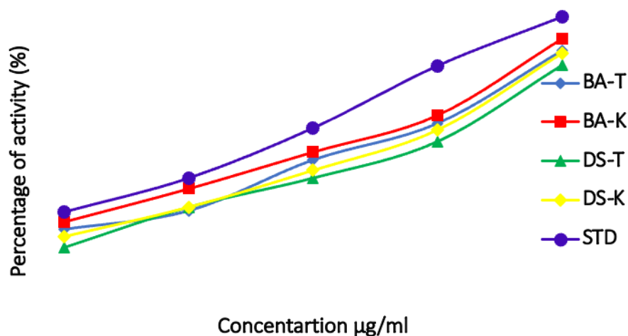
Fig.4: Hydroxyl radical scavenging activity in aqueous extract of Ba-T, Ba-K, Ds-T and Ds-K
