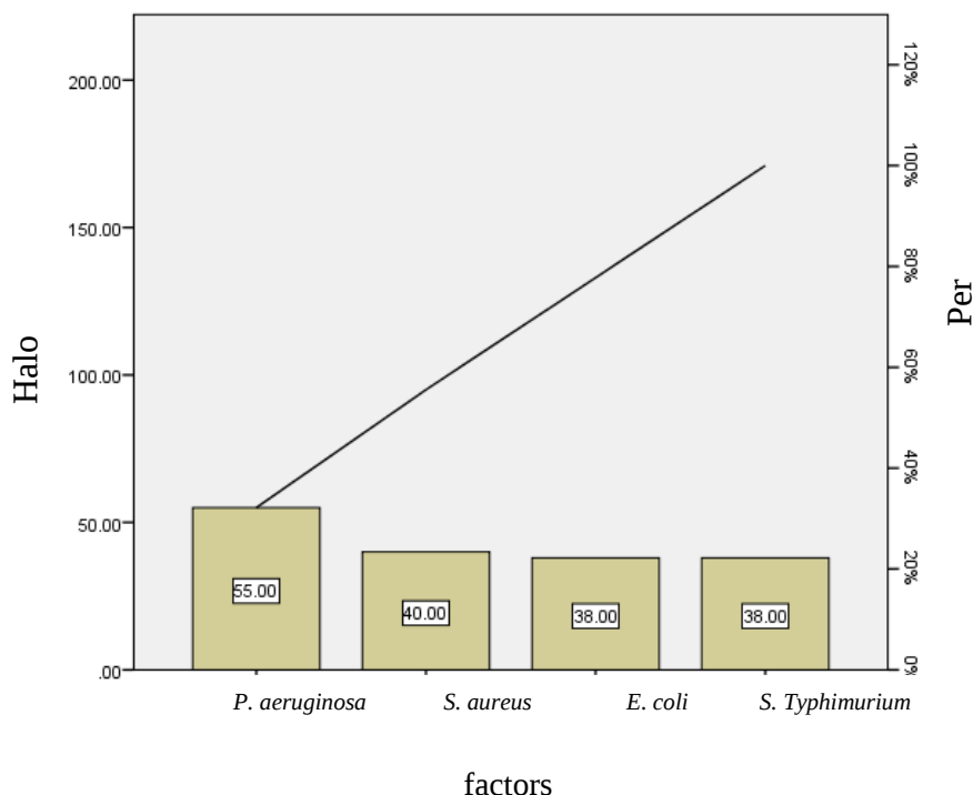
Figure 5- Prato chart (ranking) to compare the inhibitory power of L. casei total extract on pathogenic
