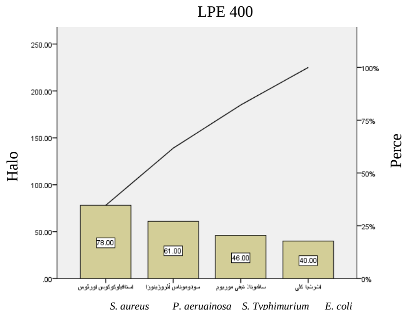
Figure 6 - Frato chart (ranking) to compare the inhibitory power of LPE 400 L. casei on pathogenic agents
