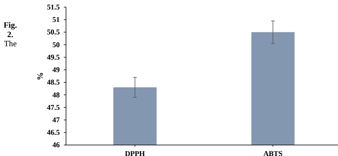
antioxidant activity (DPPH & ABTS) of Levilactobacillus brevis KKP 3945.
