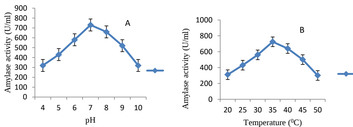
Figure 3: Effect of (a) pH (b) Temperature on \alpha -amylase production using optimized substrate (10% potato peels) after 48h of incubation.
