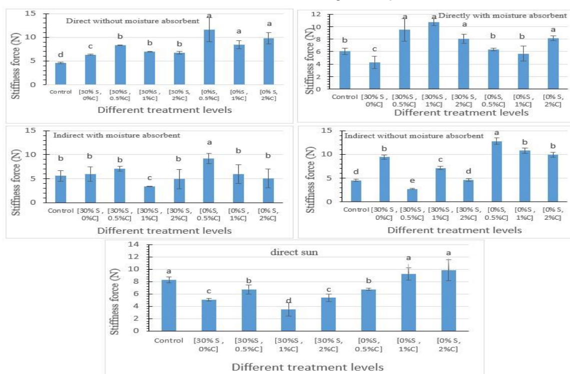
FIG 3: Changes in hardness in Newtons in apple samples dried in different concentrations of ucrose and cinnamon by direct solar drying (with and without moisture absorber), indirect (with and without moisture absorber) and traditional method ( p < 0.05 )
