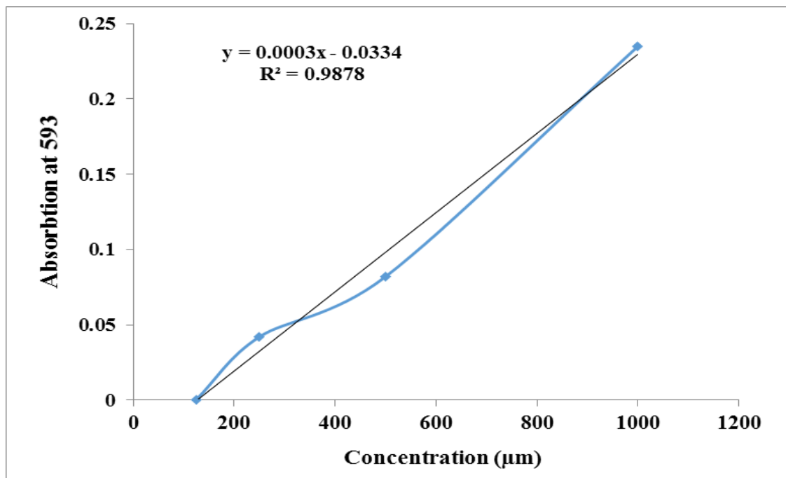
Fig.3: Calibration curve for FRAP assay
