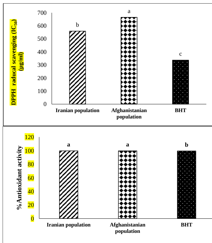
Fig.3. Antioxidant activity of Iranian and Afghanestanean populations of Ferula assa-foetida compared with BHT by DPPH (A) and \beta -carotene-linoleic acid (B) assays. Different letters indicate significant differences at P < 0.05 among treatments.
