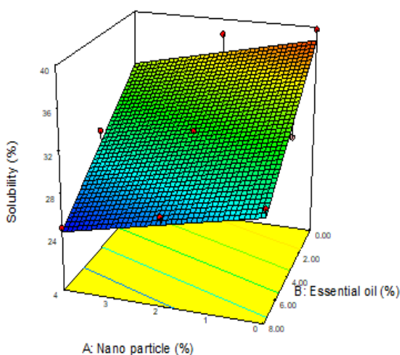
Figure 5: The three-dimensional figure of solubility of fenugreek seed mucilage film and eggplant peel powder with copper nanoparticles and rosemary essential oil.
