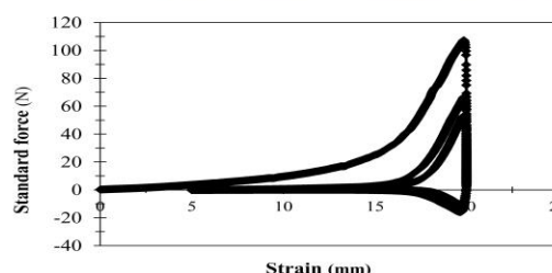
Figure 2- Material Tissue Machine, textural parameters test, An example of the force-strain diagram of the this test performed on the specimens
