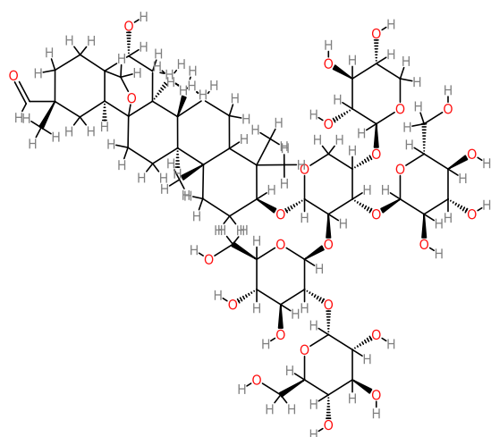
Saponin ( C_{58}H_{94}O_{27} )
