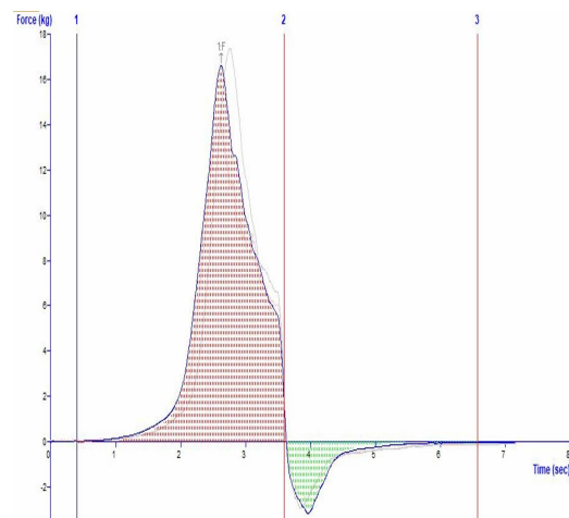
Fig 5 Kramer Texture Test Curve
