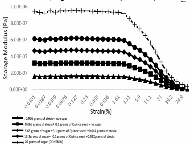
Fig 1 Storage modulus of jelly powder samples as a function of strain at 25°C and at a constant frequency of 1 Hz.
