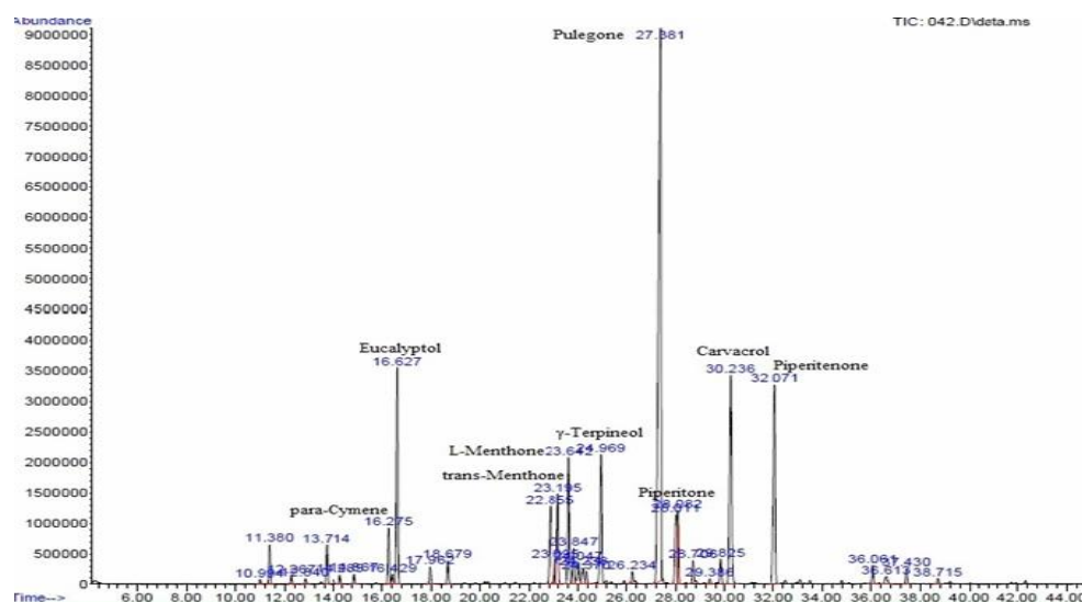
Fig 8 GC/MS analysis of Ziziphora clinopodioides essential oil.
