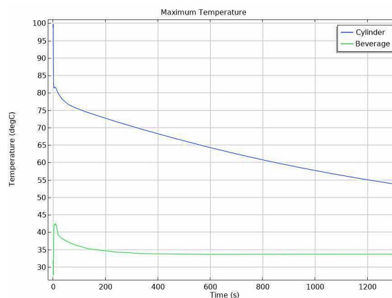
Fig 8 Simulated kinetic of temperature changes in cylinder and milk in 1200 seconds
