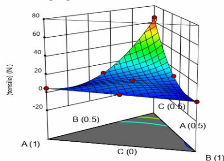
Fig 2 The effects of gelatin (A), Persian gum (B) and glycerol (C) on the tensile amount of the film.
